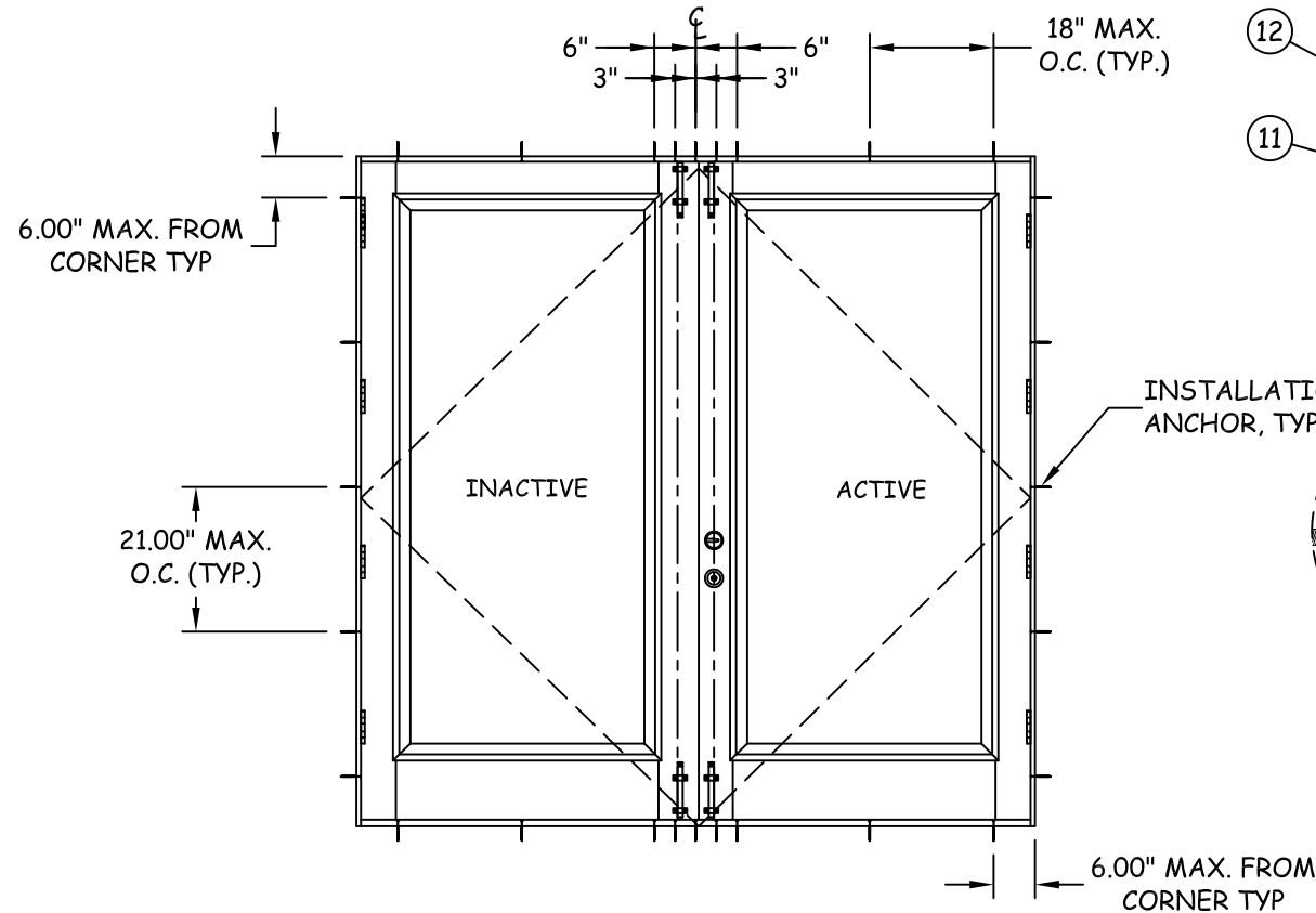
ANCHOR LAYOUT
