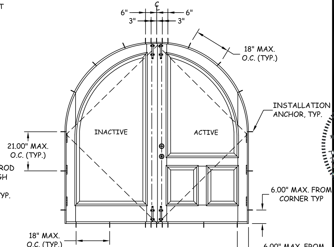
ANCHOR LAYOUT
